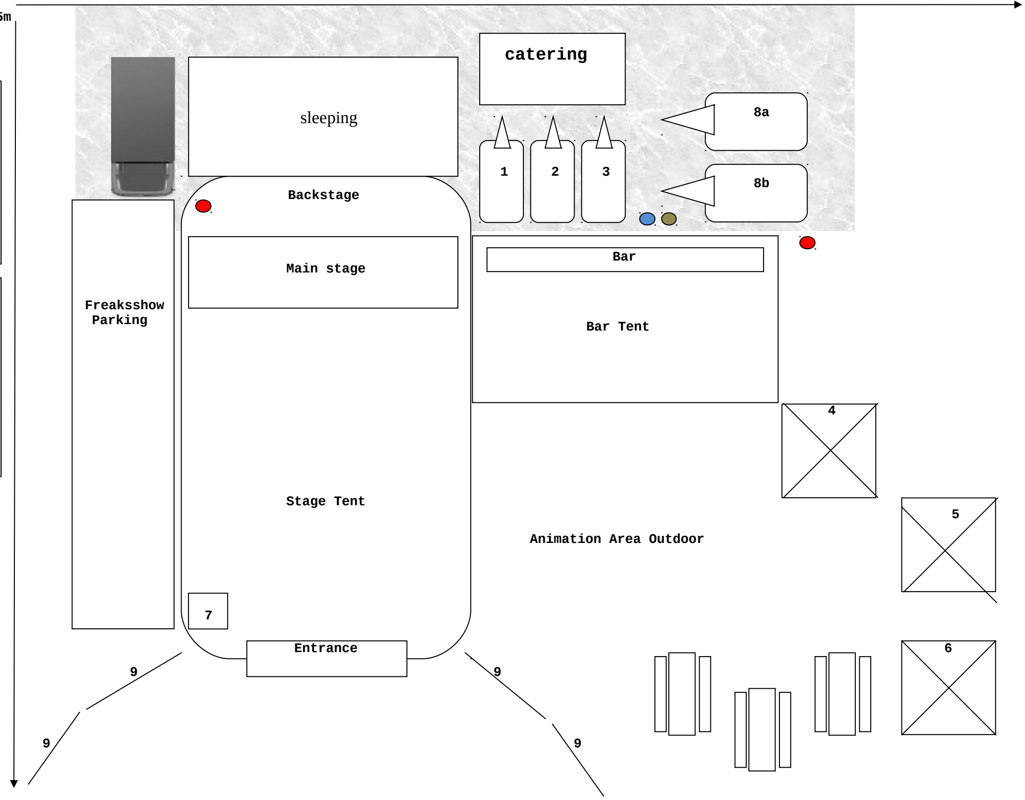
Layout Plan Freaks Show 2015
